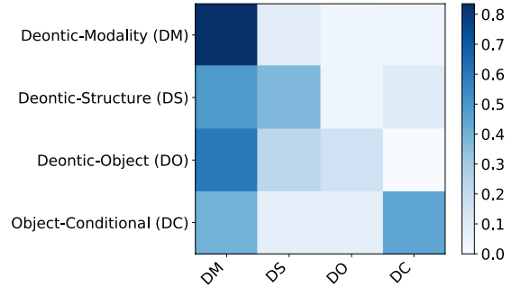
Figure 2: Confusion matrix of the TypeC ( E_{conc} ) model.
