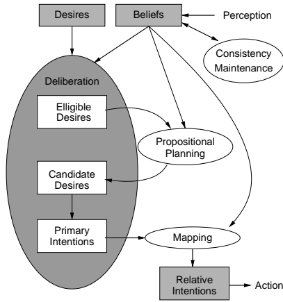
Figure 1: Modified X-BDI overview.
